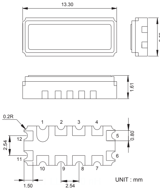
SMD 13.3 BY 6.5 SMD PACKAGE
